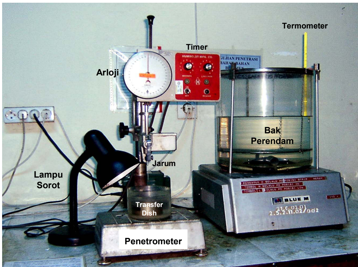
Gambar 2 - Penetrometer
